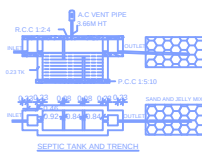
SEPTIC TANK AND TRENCH
