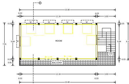
EB- ROOM FIRST FLOOR PLAN
