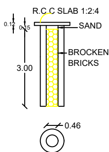
PERCOLATION PIT
