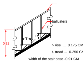
Details of staircase
