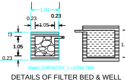
DETAILS OF FILTER BED & WELL
