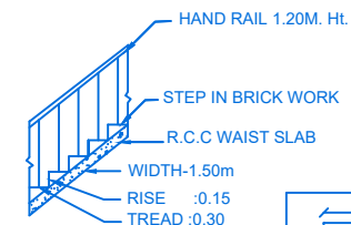
STAIR DETAIL
