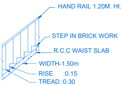
STAIR DETAIL
