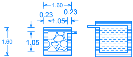
RWH_CAPACITY_L=1000LTRS DETAILS OF FILTER BED & WELL
