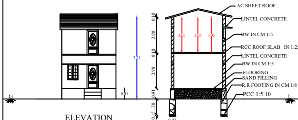
SECTION-AB&CD
