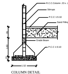
COLUMN DETAIL
