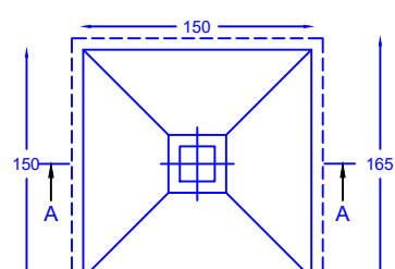
RCC FOUNDATION PLAN (SCALE 1:50)
