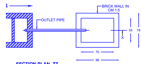
SECTION ZZ TANK AND D-TRENCH DETAILS (SCALE 1:100)
