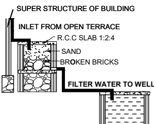
RAINWATER HARVESTING
