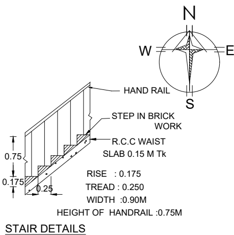
STAIR DETAILS
