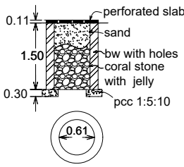
Percolation pit
