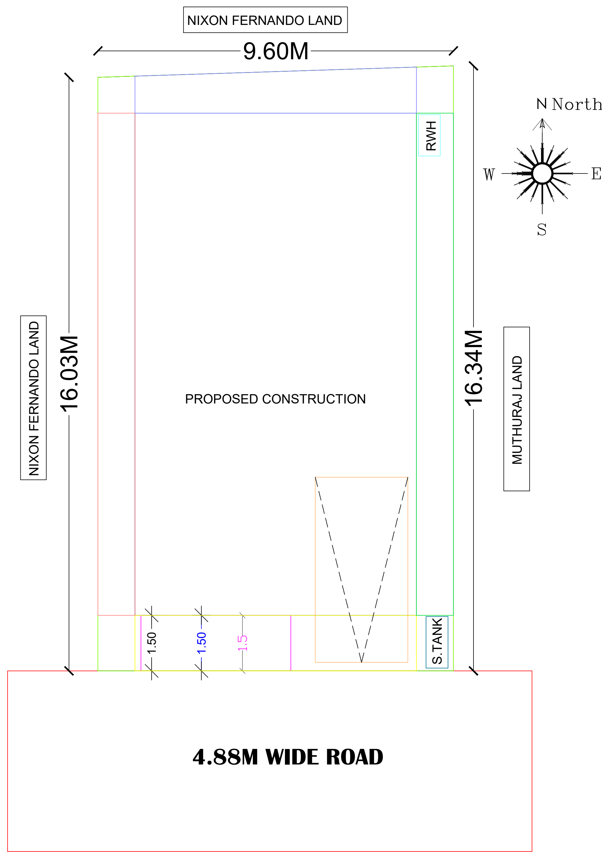
SITE PLAN
