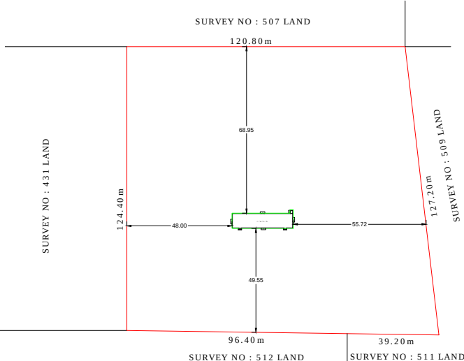
SITE PLAN (SCALE :- 1:800)
