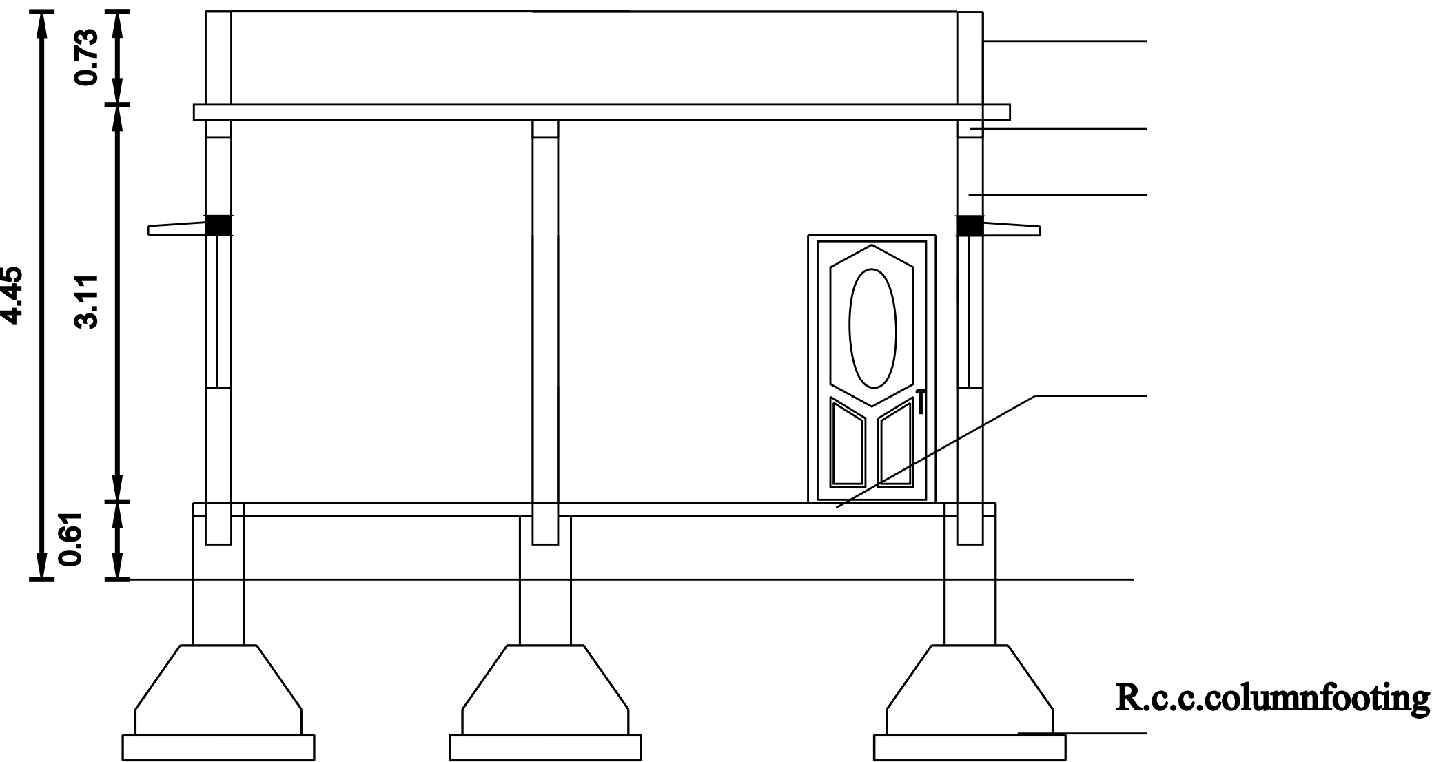
SECTION-AA
