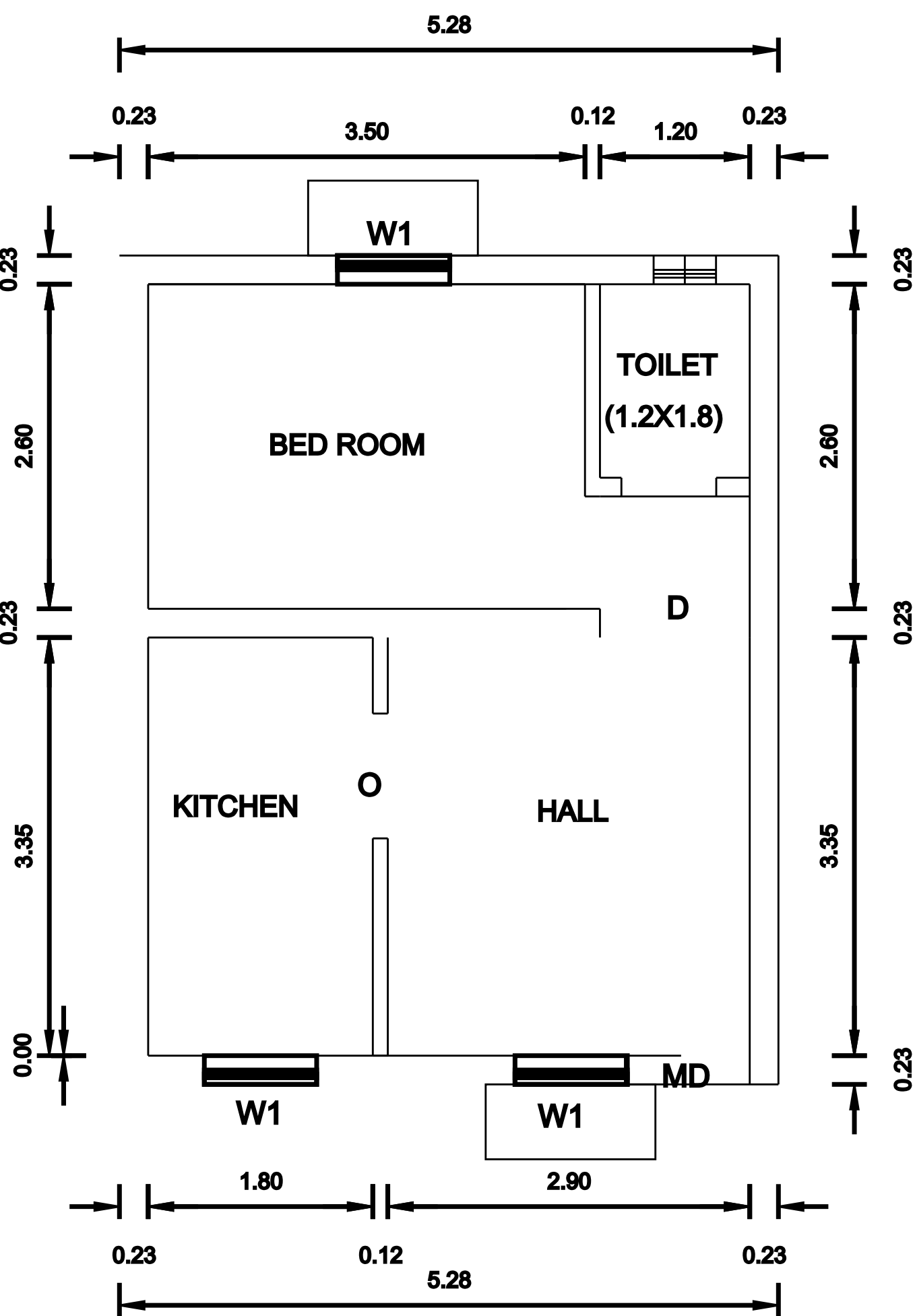
PLAN
