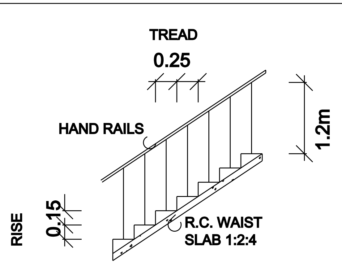
STAIRCASE DETAILS
