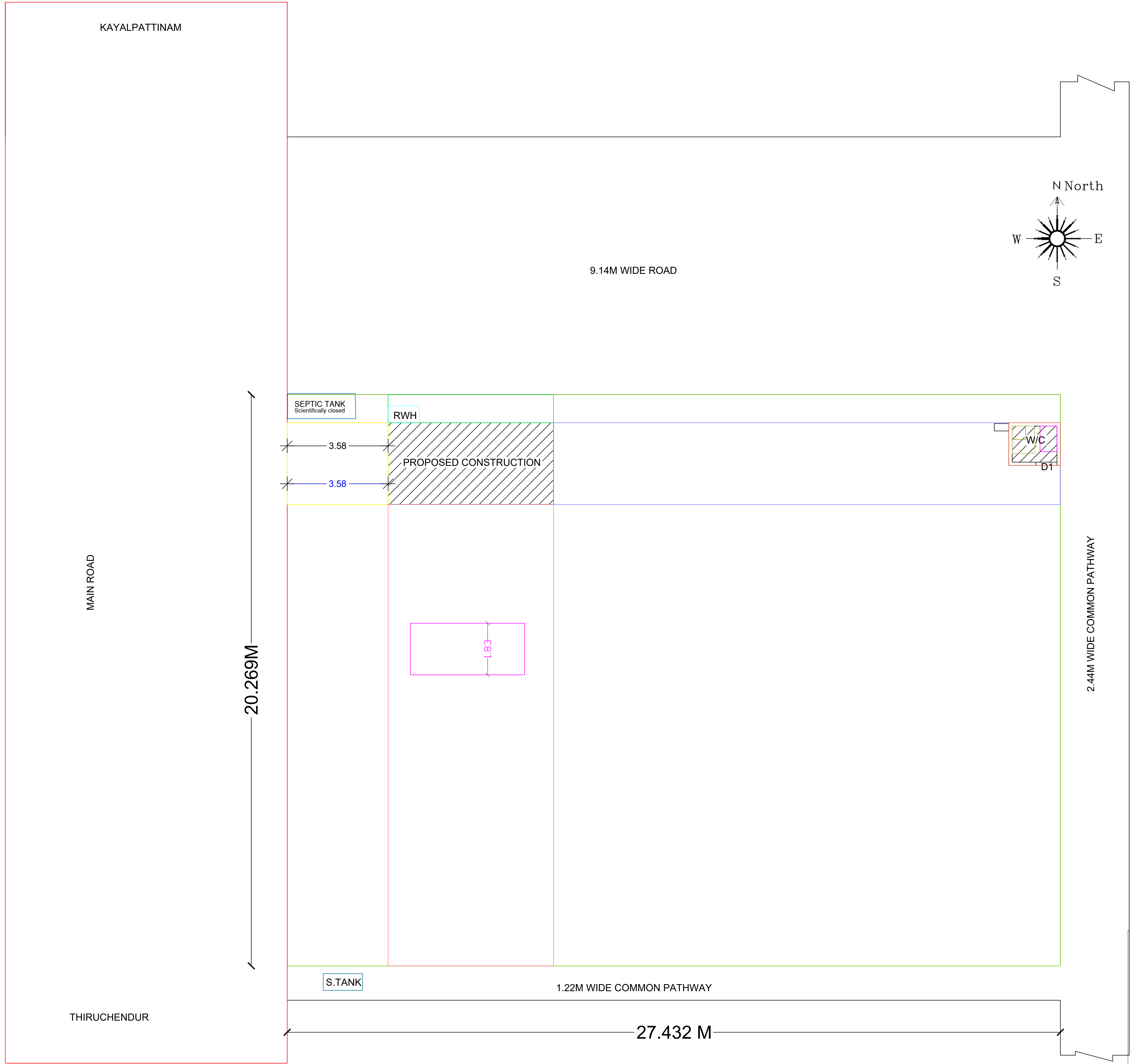
SITE PLAN
