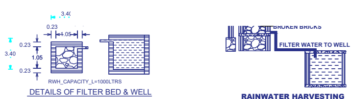
DETAILS OF FILTER BED & WELL
