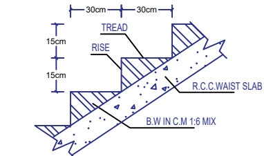
STAIRCASE DETAILS
