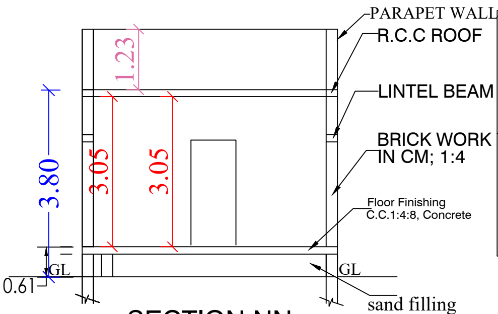
SECTION NN
