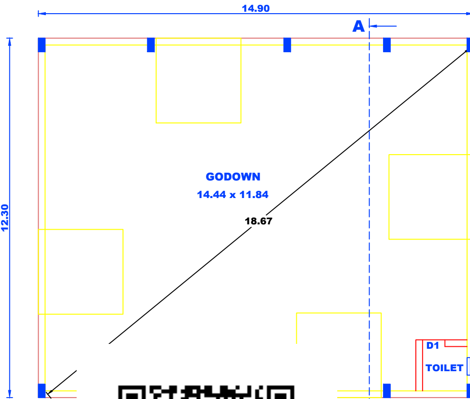
PLAN
