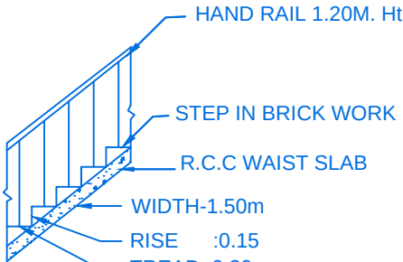
STAIR DETAIL
