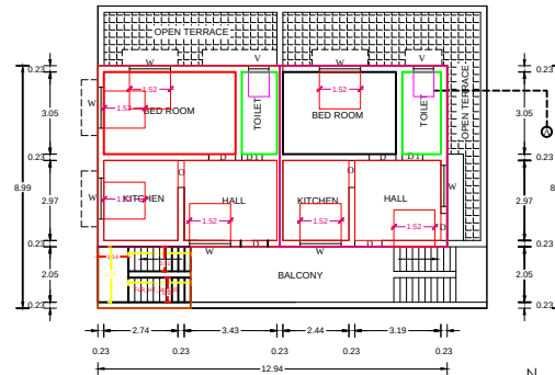
PRO SECOND FLOOR PLAN
