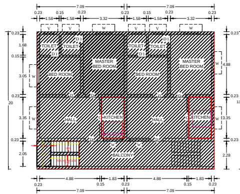
EXG.FIRST FLOOR PLAN
