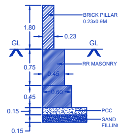
FOOTING DETAILS
