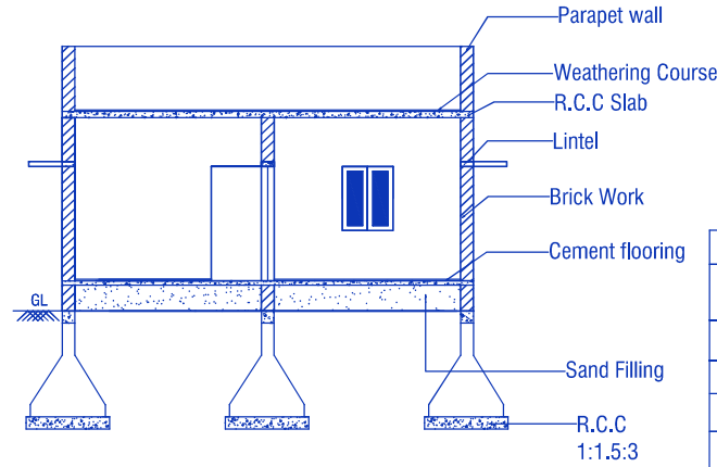
CROSS SECTION ON 'A-B'
