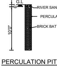
PERCOLATION PIT
