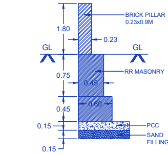
FOOTING DETAILS
