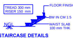
STAIRCASE DETAILS
