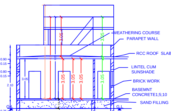
SECTION AB
