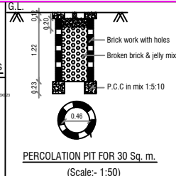
PERCOLATION PIT FOR 30 Sq. m.
