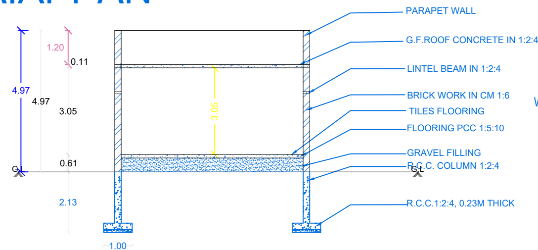
SECTION ON-AA
