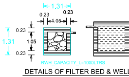
DETAILS OF FILTER BED & WELL
