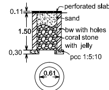
percolation pit
