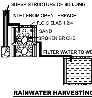
RAINWATER HARVESTING
