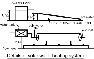
Details of solar water heating system
