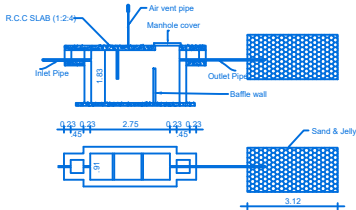
SEPTIC TANK & TRENCH
