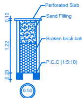
RAIN WATER COLLECTION WELL
