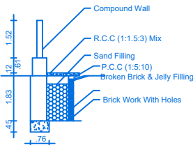
RAIN WATER HARVEST DETAILS
