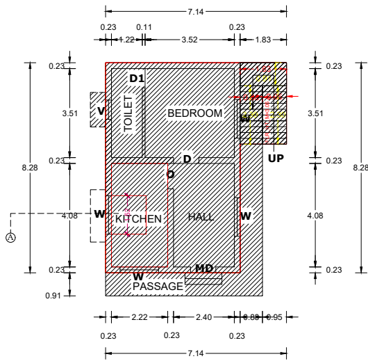
EXG.GROUND FLOOR PLAN
