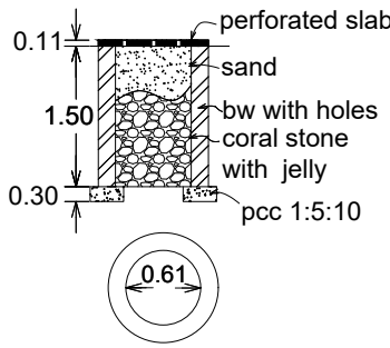
percolation pit
