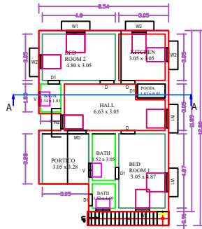
PLAN LAYOUT
