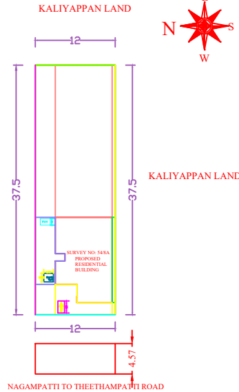
SITE PLAN
