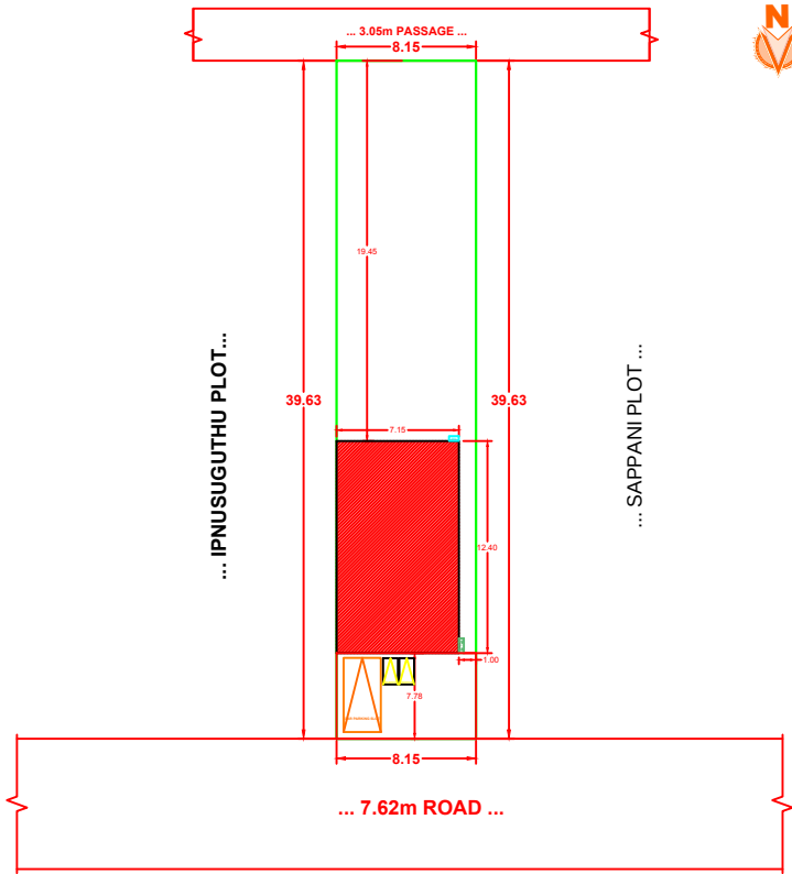
SITE PLAN FOR THE PROPOSED BUILDING SCALE: 1:200
