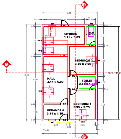
GROUND FLOOR PLAN FOR THE PROPOSED BUILDING
