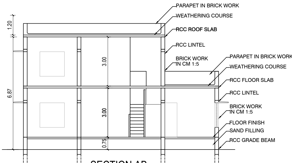
SECTION AB
