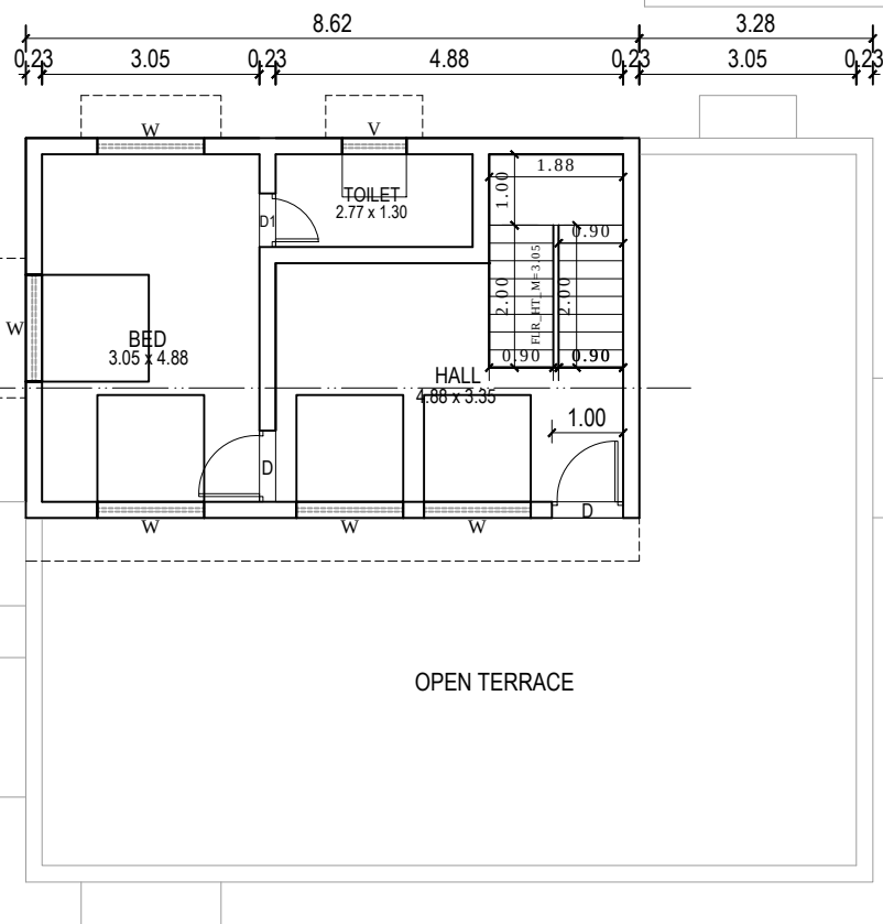
FF PLAN
