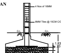
BCC COLUMN DETAILS
