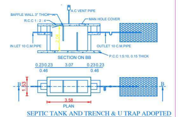
SEPTIC TANK AND TRENCH & U TRAP ADOPTED
