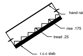
STAIR
