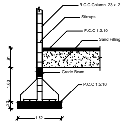
COLUMN DETAIL
