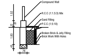
RAIN WATER HARVEST DETAILS
