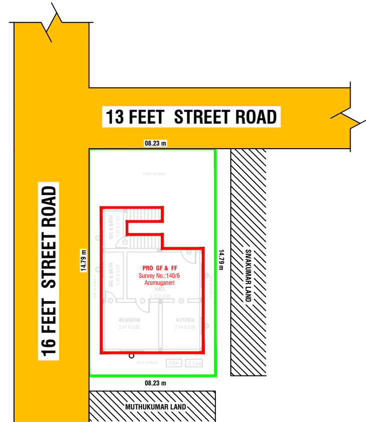
SITE PLAN (1:100)
