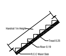
STAIR DETAILS
