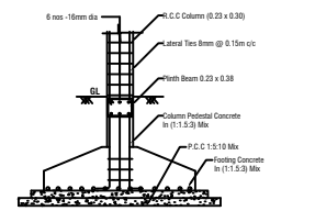
COLUMN FOOTING DETAILS
