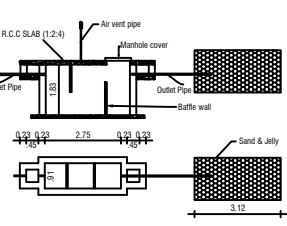
SEPTIC TANK & TRENCH
