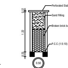
RAIN WATER COLLECTION WELL
