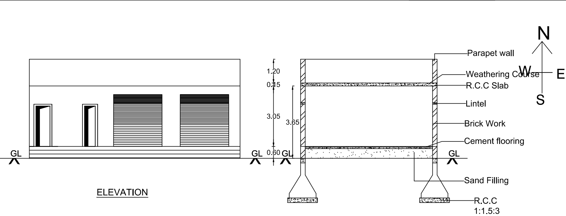
CROSS SECTION"AA"
