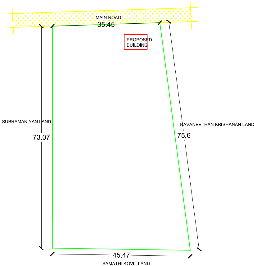
SITE PLAN
