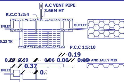
SEPTIC T
