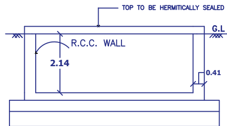
RWL SECTION (SAMPLE) RWL_CAPACITY_L=2000LTRS
