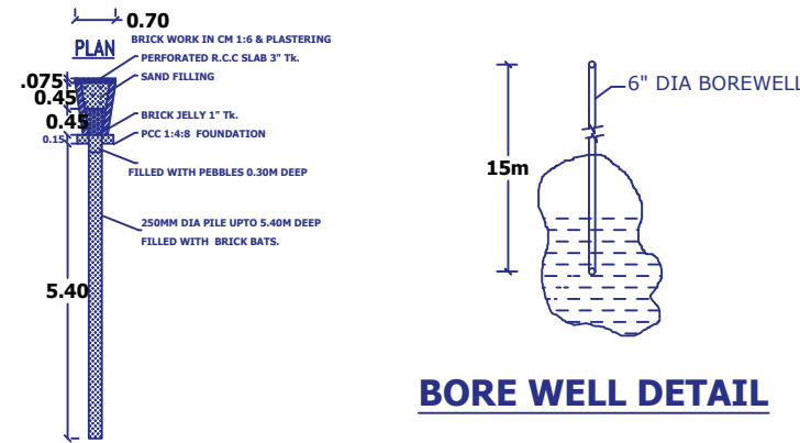
PERCOLATION PIT
