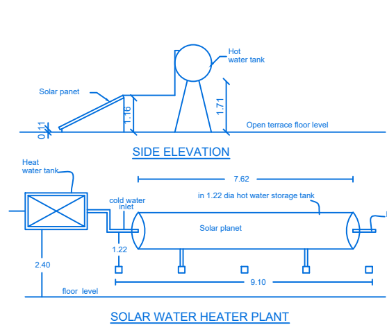
SOLAR WATER HEATER PLANT
