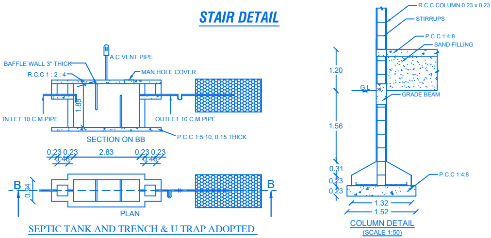
SEPTIC TANK AND TRENCH & U TRAP ADOPTED
