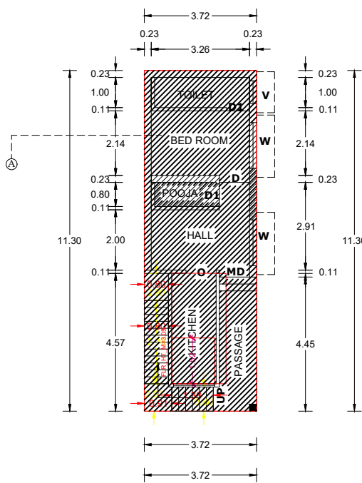
EXG.GROUND FLOOR
