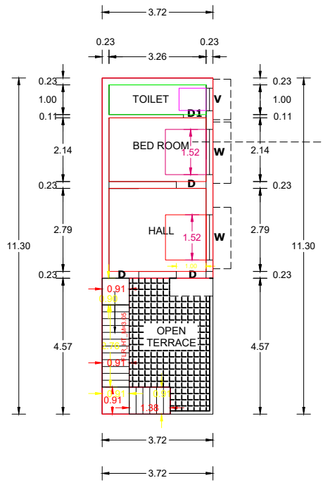
PRO.FIRST FLOOR
