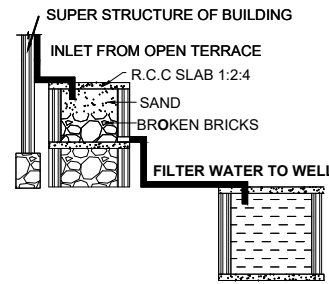
RAINWATER HARVESTING
