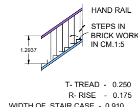
DETAILS OF STAIRCASE
