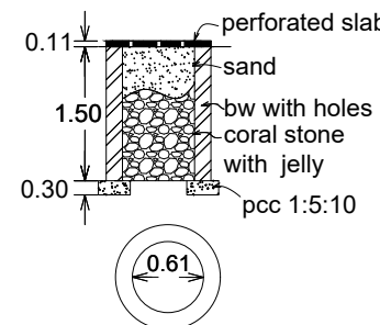
percolation pit
