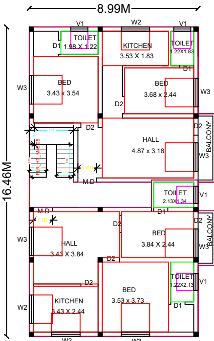
FIRSTFLOOR PLAN
