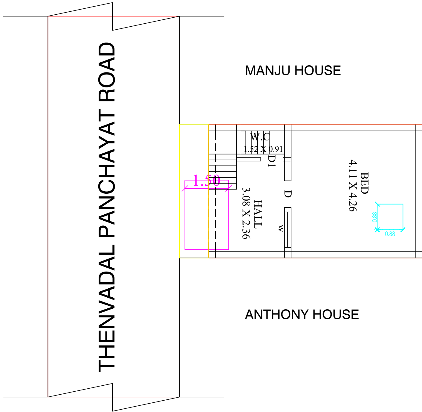
SITE PLAN
