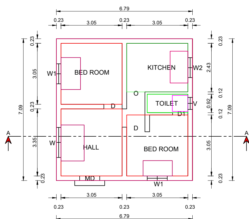
GROND FLOOR PLAN
