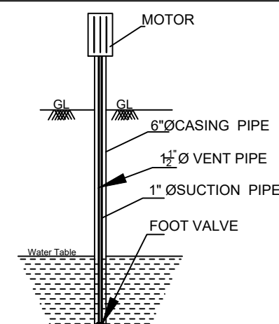
SEC. OF BOREWELL
