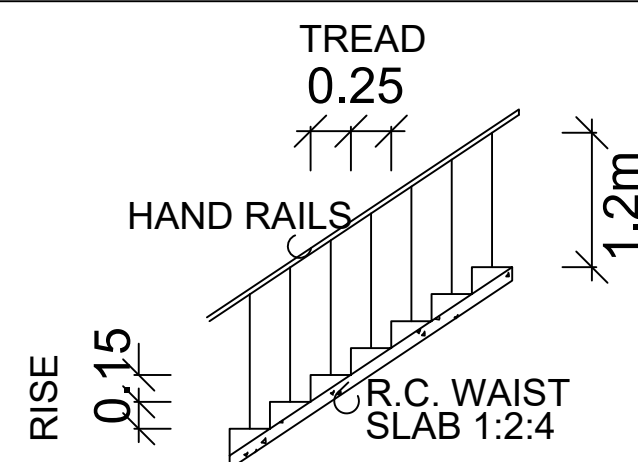
STAIRCASE DETAILS
