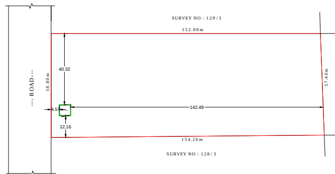
SITE PLAN
