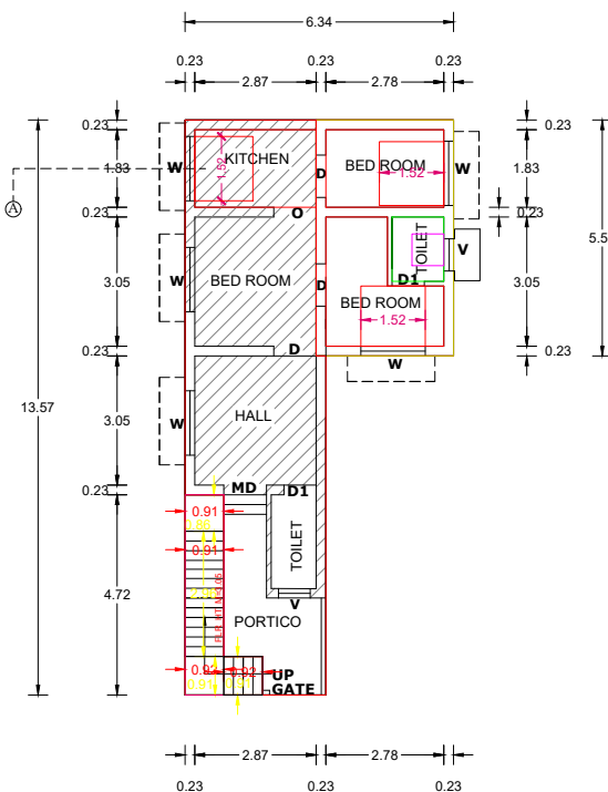
EXG. & PRO. GROUND FLOOR PLAN
