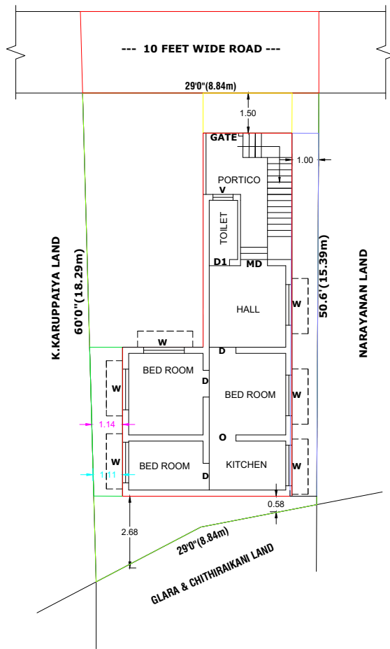
SITE PLAN
