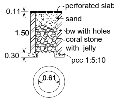
percolation pit
