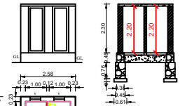
BLK-2 BATH ROOM PLAN
