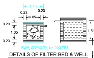
percolation pit
