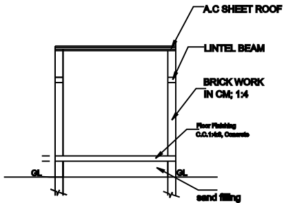
SECTION NN
