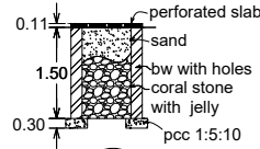
percolation pit
