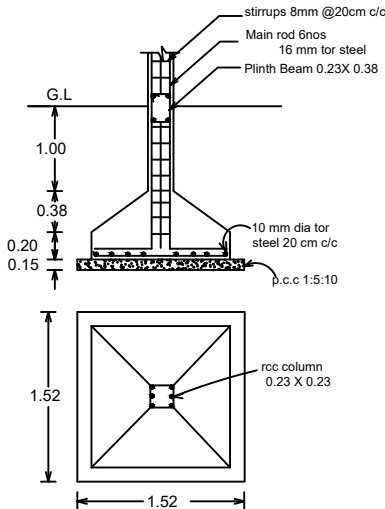
Details of COLUMN
