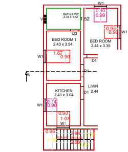
PROPOSED GROUND
